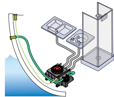
Grey Water Tank with Viking Power 16
